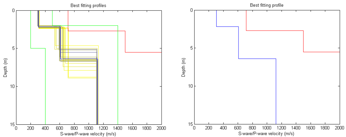
Figure 7 Varese Ligure – a) Monte Carlo results (from yellow to blue) of the inversion with the boundaries (green) compared with the refraction result (red). b) Varese Ligure – Best fitting profile (blue) compared with the refraction result (red).
