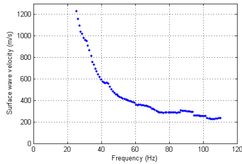
Figure 6 – Varese Ligure -Average apparent dispersion curve
