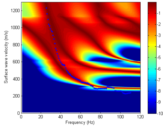
Figure 8 Varese Ligure – Experimental dispersion curve compared with the misfit surface of the best fitting model
